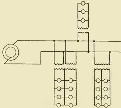
Fig. 15. Single-Phase System with Secondary 3-Wire System
